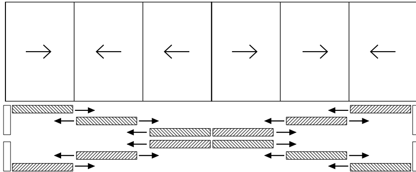
Manually operated - 6 sashes
